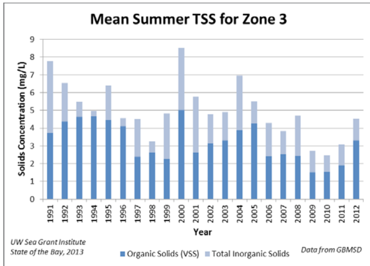
Figure 18: Graph of mean total suspended solids concentrations for zone 3.
