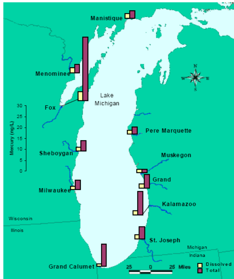
Figure 40: Mean total and dissolved mercury concentrations measured in Lake Michigan tributaries (map from the EPA 2004).
