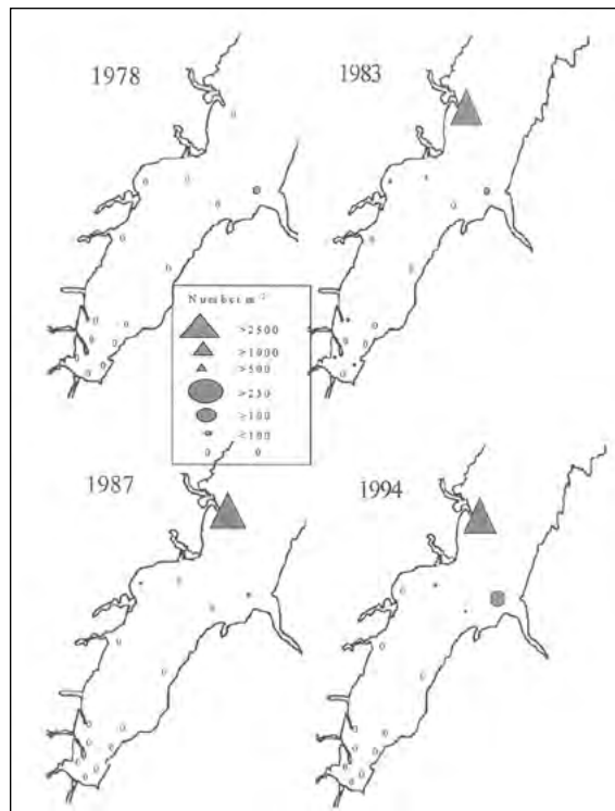
Figure 62: Comparison of the distribution of the amphipod, Diporeia . From Fettes, 2001.
