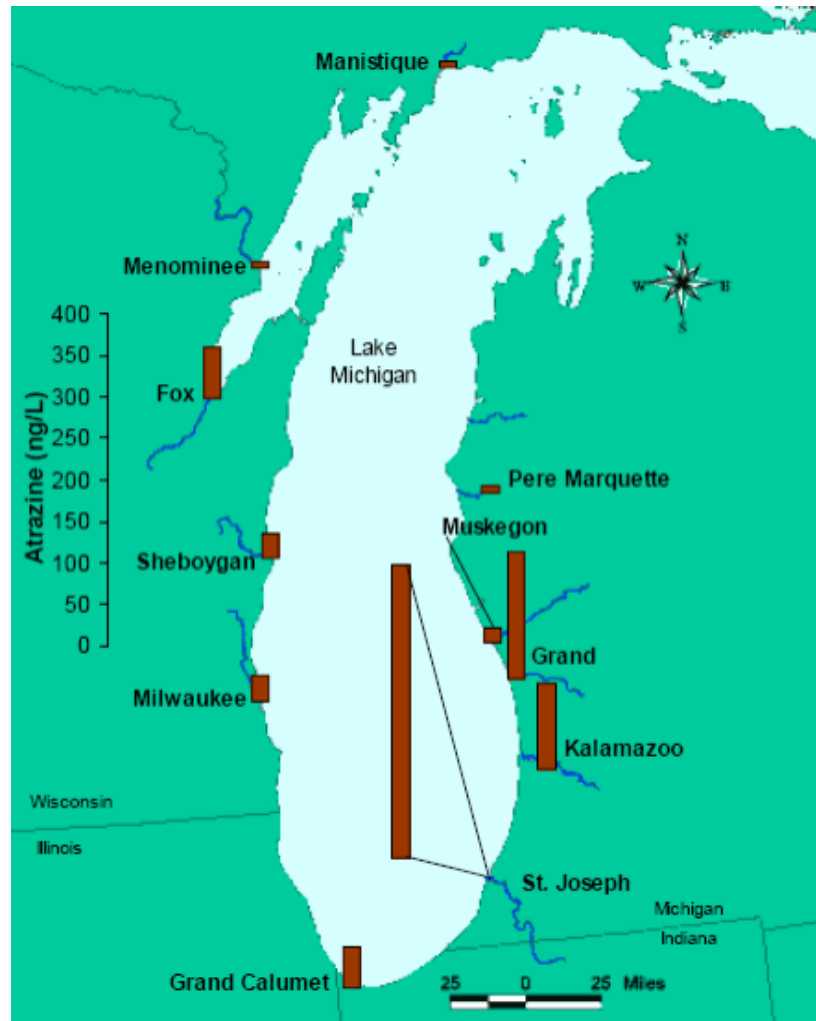
Figure 44: Mean atrazine concentrations measured in Lake Michigan tributaries (map from the EPA 2001).
