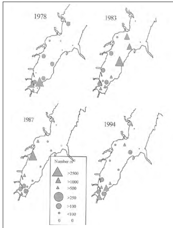
Figure 60: Comparison of the distribution of chironomids. From Fettes, 2001.
