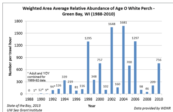
Figure 83: Relative abundance of YOY white perch as measured by number per trawl hour from data collected in annual late summer trawl surveys for years 1988-2010. Data provided by the WDNR.
