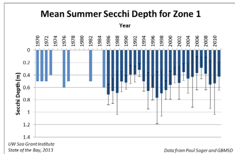
Figure 24: Graph of mean Secchi depths for zone 1. The error bars represent one standard deviation. Dr. Sager provided data from 1970-1985 (light blue bars) and GBMSD provided 1986-2011 data (dark blue bars).
